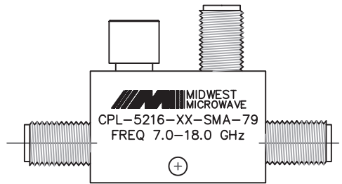
BACKSIDE MARKING
