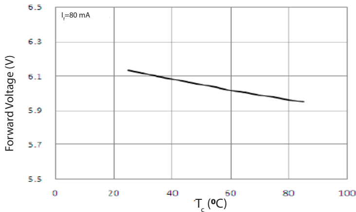
Tc--Forward Voltage
