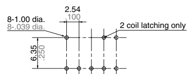
PC board pattern (Bottom view)
