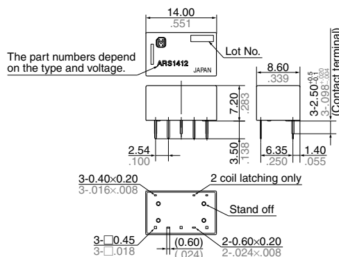
External dimensions
